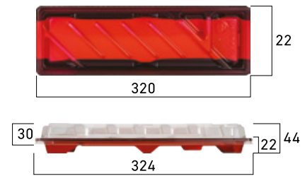
뚜껑 Cap Code: P211214-MPA
