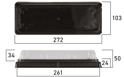
뚜껑 Cap Code: P160609-MPA
