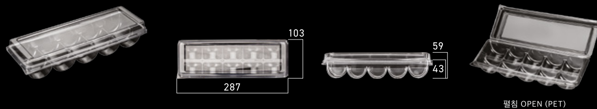
펼침 OPEN (PET)
