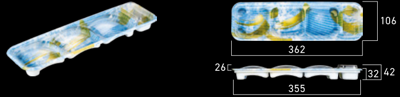
DESIGN 특허 DRE-SASHIMI-29 DRE-회29 Patent No : 30-2019-0045884 362×106×42(SET)
