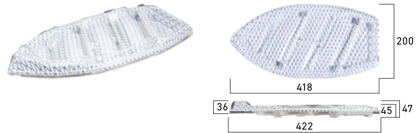
DR-SASHIMI BOAT-2-1 DR-선(船)-2-1 Patent No : 30-2022-0030895 422×210×47(SET)
